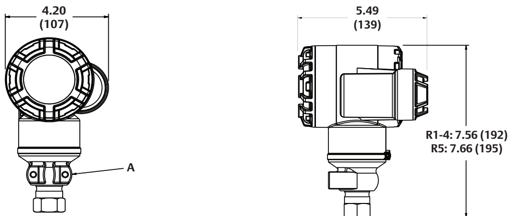
Figure 10. 3051T Wireless Housing Dimensional Drawings
