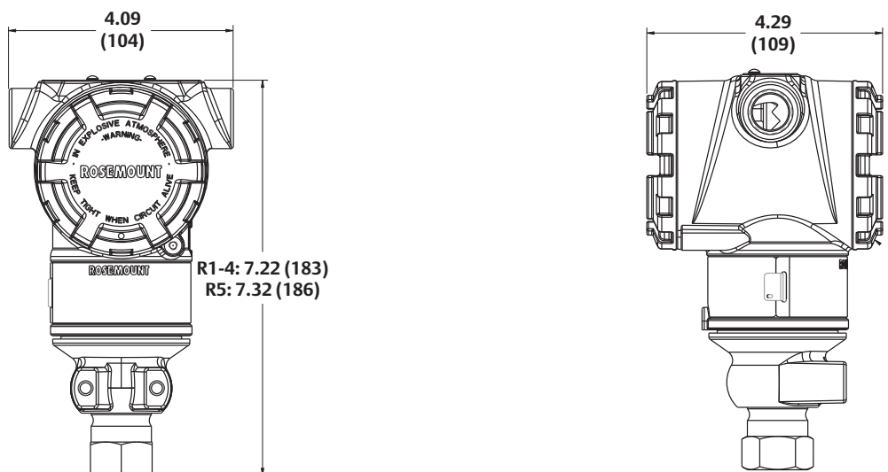
Figure 10. 3051T Wireless Housing Dimensional Drawings
